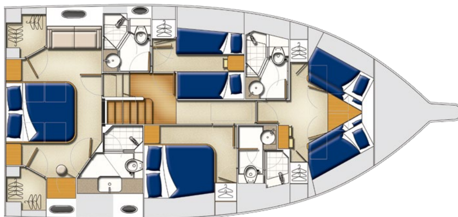
Optional starboard guest VIP cabin with double bed
